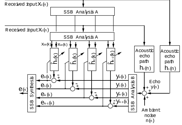
Figure 2: Proposed subband stereo echo canceller.
