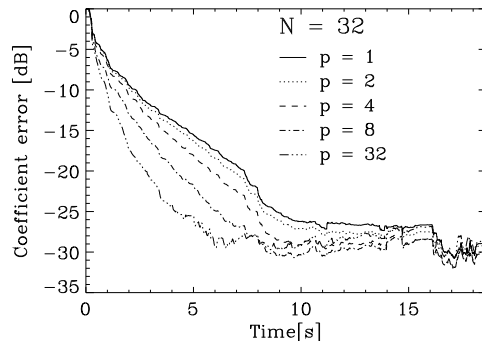
(a) Coefficient error
