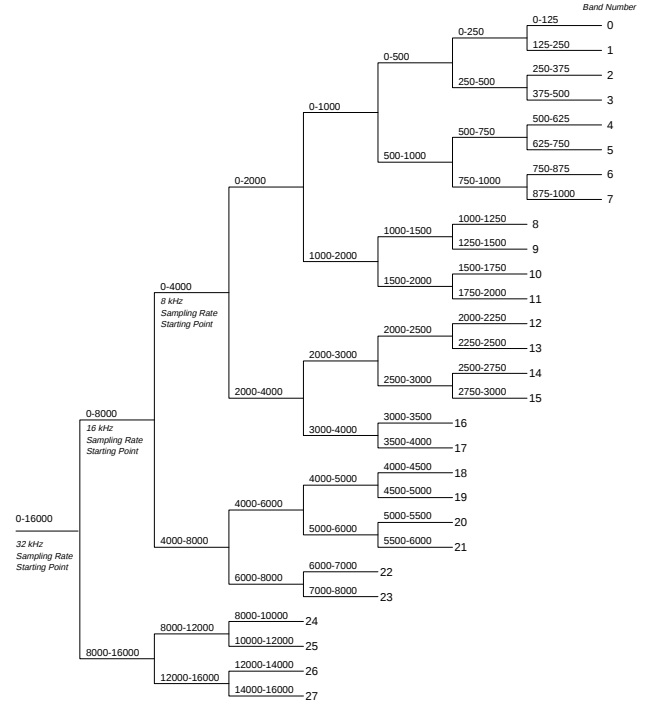
Figure 2: WP Tree Structure for 32kHz, 16kHz, 8kHz Sampling Rates
