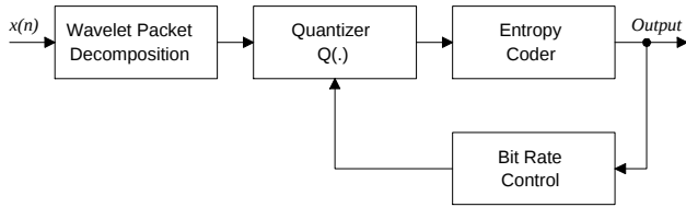
Figure 1: Encoder Block Diagram
