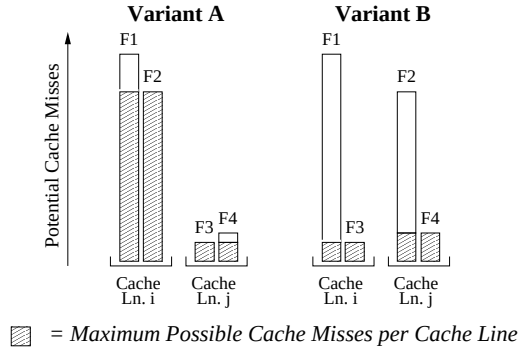
Figure 3. Two variants of function overlapping in cache lines.
