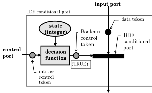
Fig. 2 IDF dataflow control
