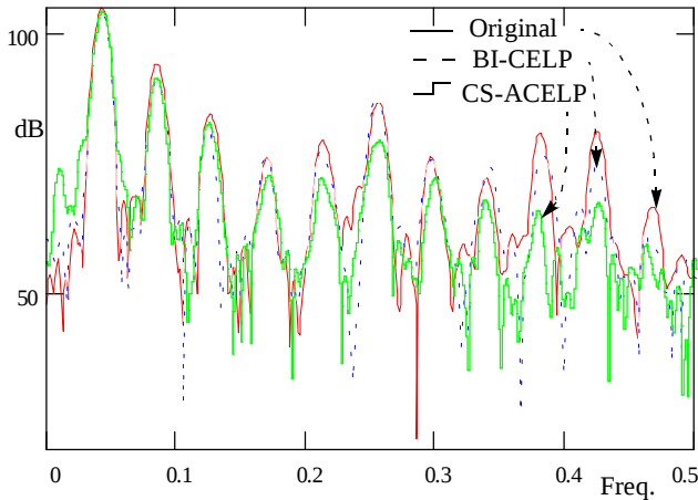
Fig. 4 Output Spectrums of BI-CELP and CS-ACELP
