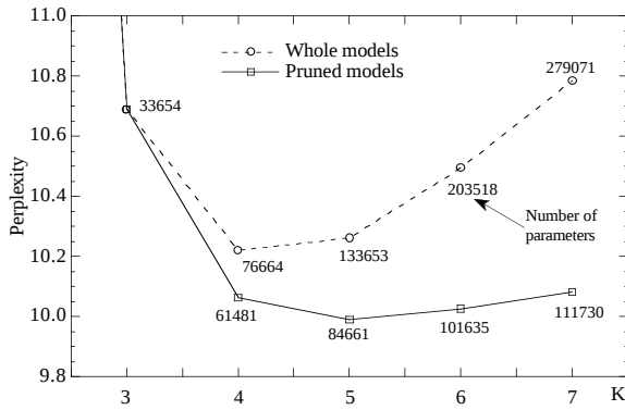
Figure 6. For any value of K, the best model is obtained after pruning. This effect allows, for a similar size, an increase in the value of K and an improvement in the performance by means of deleting some low-k states and including some more significant higher-k states.
