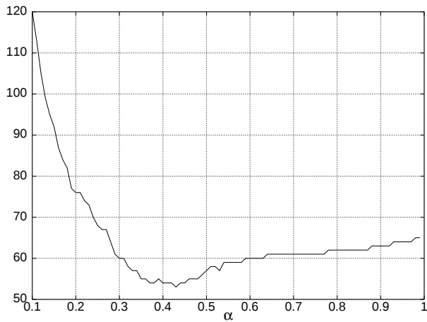
Figure 1: Errors for the digits task as a function of \alpha
