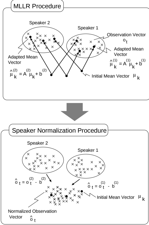
Figure 1. An example of normalizing observation vectors using MLLR.
