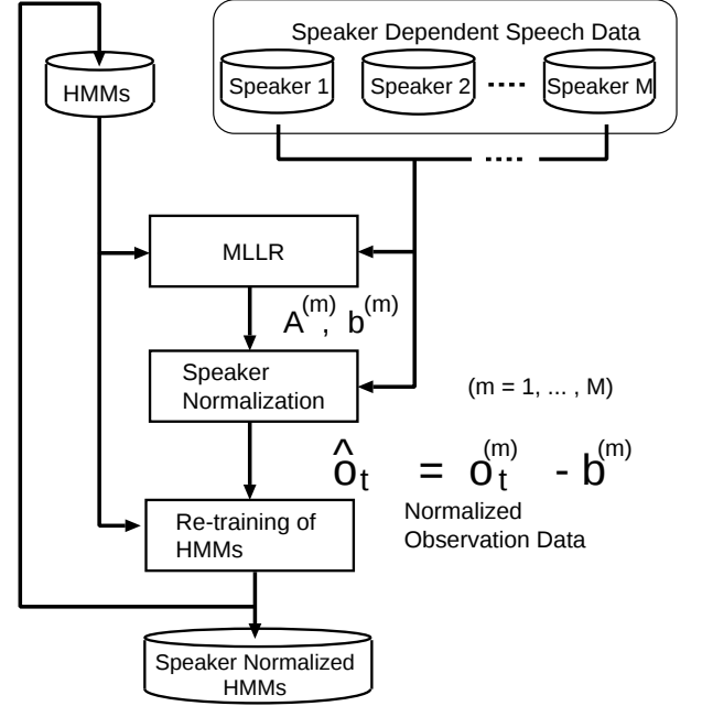
Figure 2. Procedure for generating a normalized speaker independent model.
