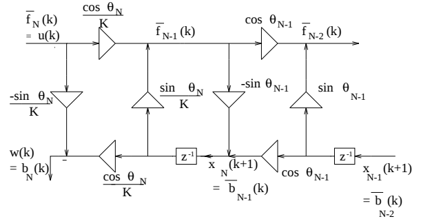
Figure 1. Modified normalized lattice filter; the parameters are time-varying.
