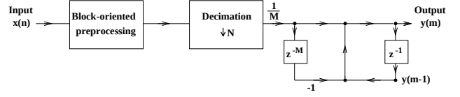
Figure 2. Block-recursive sliding-window averager scheme, n = mN , window-size: MN
