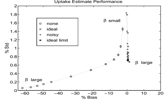
Figure 4: Comparison of empirical standard deviation vs. bias for no, ideal, and noisy (ML extracted) side information.
