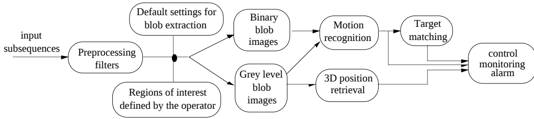
Figure 1. The harbour control system block diagram.
