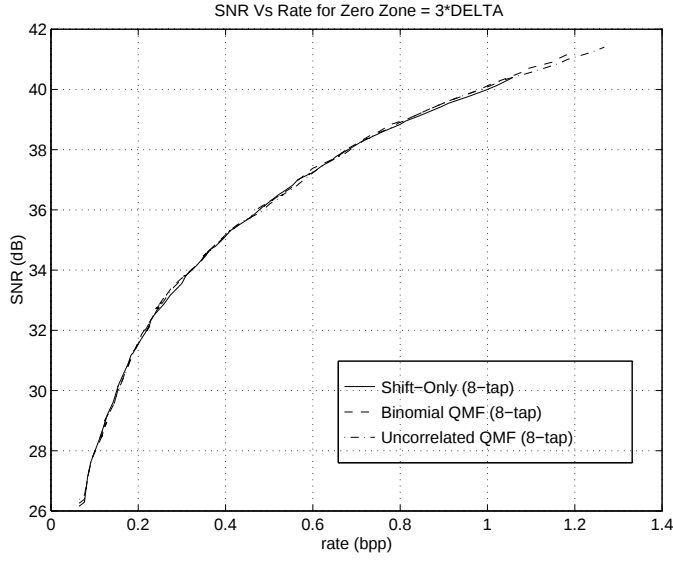
Figure 1: Rate - Distortion Performance Curves for different filter families with zero zone = 3 \cdot \text{DELTA} .
