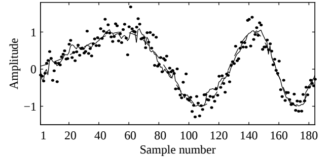
Figure 2: Test input (dotted) with SNR of 10 dB and maximum frequency of 10 Hz, and target output (dashed) sweeping sinusoidal signal, along with the NN1 output signal (solid).
