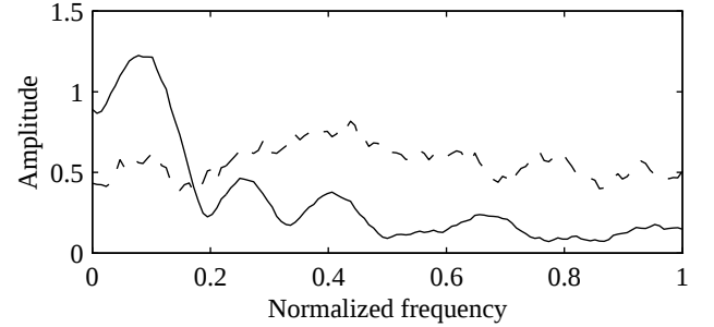
Figure 4: Welch method frequency response estimates of the NN1 (solid) and NN4 (dashed).
