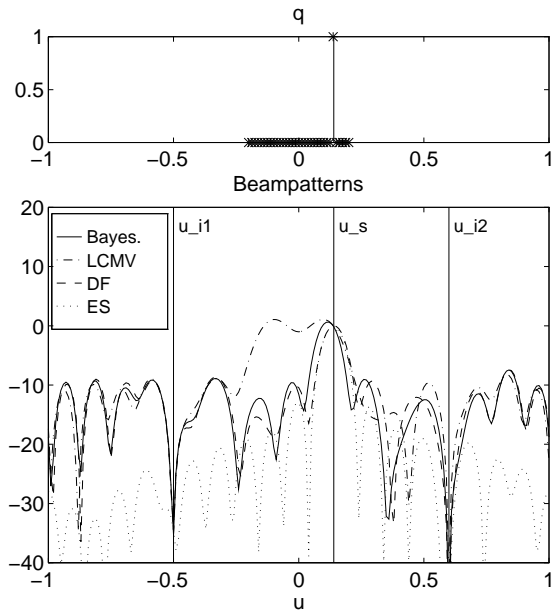
Figure 1: p(u) and beam patterns of adaptive beamformers for N=20 element ULA. The desired signal is at u_s = 0.14 with SNR = 0 dB and the interferers are at u_{i1} = -0.5 and u_{i2} = 0.6 with INR = 20 dB. A priori interval = [-0.2, 0.2] . Number of snapshots K = L = 100 .
