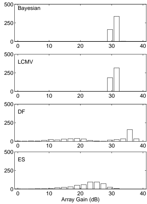
Figure 4: Same as Figure 2 with SNR = -20 dB.
