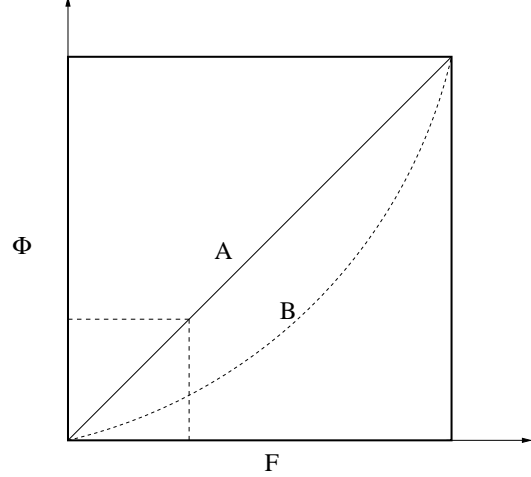
Figure 1: Continuous Lorenz Curve
