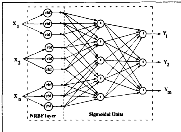
Figure 2. NRBF architecture
