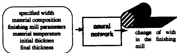
Figure 5. A neural network can improve the accuracy of the predicted lateral flow in a steel rolling mill by 1 mm.
