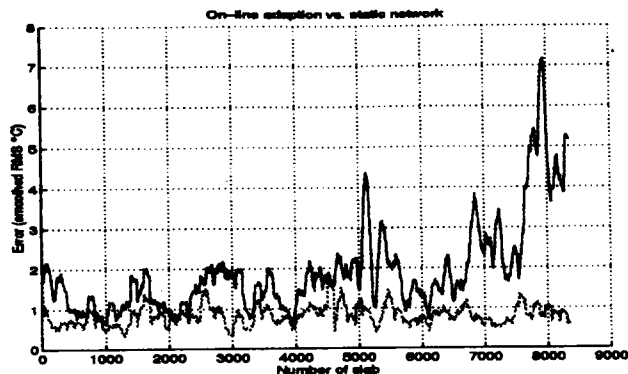
Figure 7. Without on-line adaptation after a few days the error in temperature prediction increases considerably.
