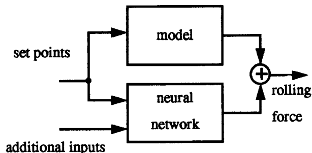
Figure 6. a hybrid system of neural net and conventional model.
