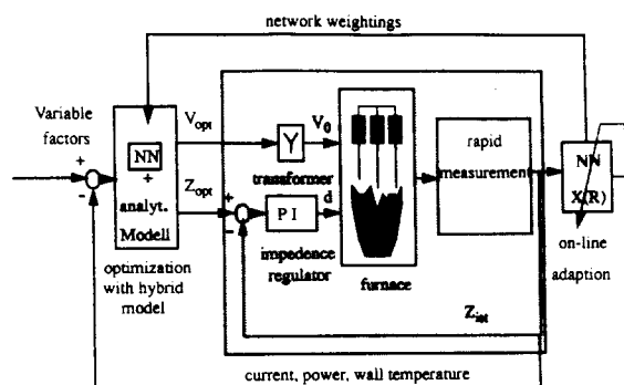
Figure 2. This hybrid model optimizes the operation of an electric arc furnace under constantly changing conditions.
