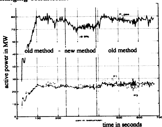
Figure 3. Neural network-derived optimization increases active power of the smelting process while satisfying all boundary conditions
