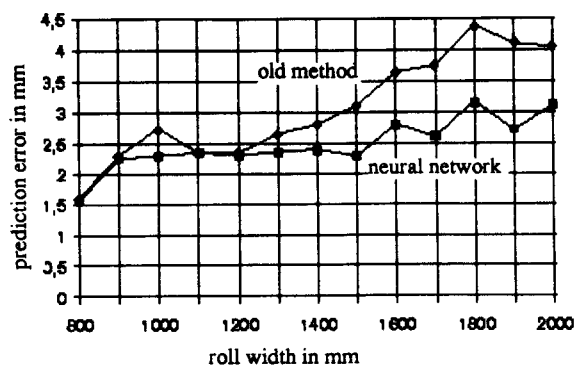
Figure 4. Predicted lateral flow error in one of Thyssen's rolling mills
