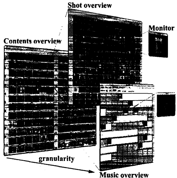
Figure 2. VideoBrowser
