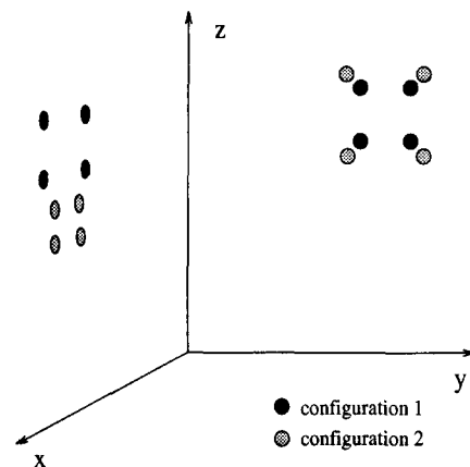
Figure 2. Microphone array arrangement for the two configuration used in the experiments.
