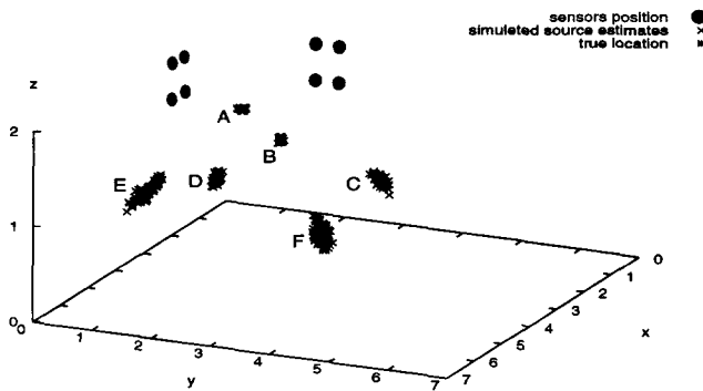
Figure 3. Distribution of source location estimates around the true position for sources at the six points evidenced in Figure 1, when TDOA estimates are all affected by gaussian noise with equal distribution.
