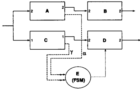
Figure 1. scheduling problem
