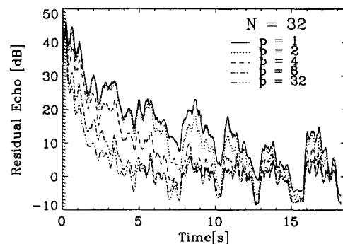
(b) Residual echo
