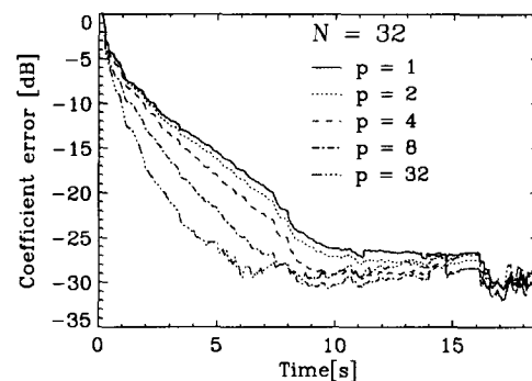
(a) Coefficient error
