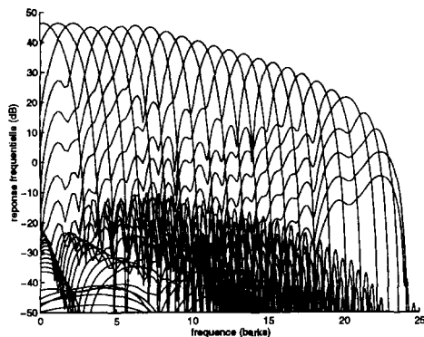
Figure 1. Frequency responses of the filters used for the "ear transform", E^k(z) (1 filter out of 2 is represented)
