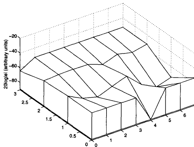
Figure 5. Error signal levels at the sensors after minimisation of the maximum value (MINI-MAX). The horizontal axes represent the row number (0 to 3) and the column number (0 to 7) of the sensors in the microphone array.
