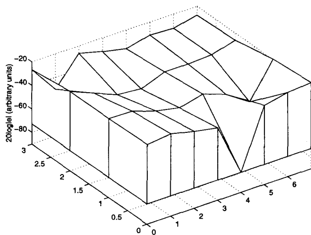
Figure 3. Original error signal levels at the sensors. The horizontal axes represent the row number (0 to 3) and the column number (0 to 7) of the sensors in the microphone array.
