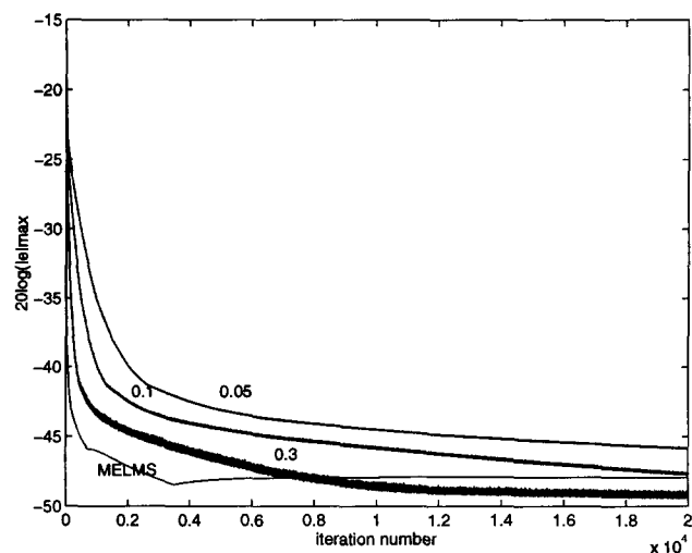
Figure 6. Evolution of the maximum error signal level for the MINIMAX algorithm with increasing values of the convergence parameter, \alpha = 0.05, 0.1, 0.3 , and for the MELMS algorithm with the maximum allowed convergence parameter.
