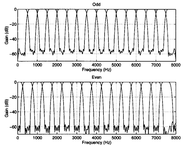
Figure 2. Frequency response of filter bank channels for odd and even channel stacking arrangements.
