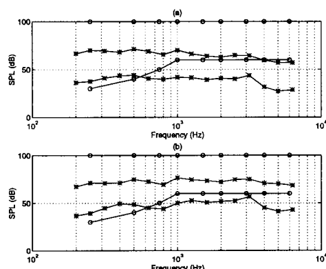
Figure 6. Mapping of 10% and 90% speech spectrum levels (*) into the residual dynamic range (O) for (a) overall level control and (b) 97% channel level control.
