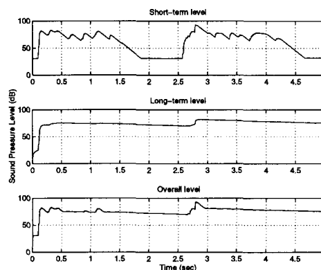
Figure 5. Level measurements versus time for a loud transient in speech showing short-term level, long-term level and the fuzzy detector "Overall" level.
