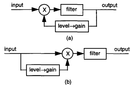
Figure 1. Basic topologies for compression systems: (a) feedback and (b) feedforward.
