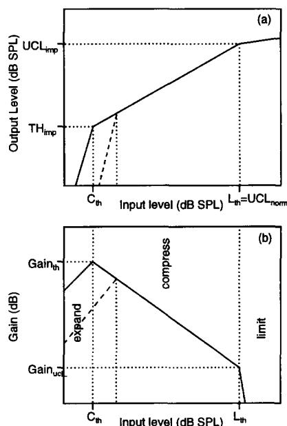
Figure 3. Static characteristics showing input versus output (a) and input versus gain (b).
