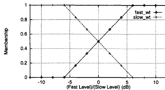
Figure 4. Fuzzy membership functions for transient (fast weight) and non-transient (slow weight) signals.
