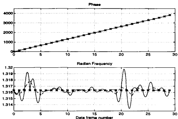
Figure 1: Interpolated frequency tracks obtained from the cubic interpolation algorithm (solid line) and the proposed quadratic interpolation algorithm (dotted line) for a special case where the frequency (stars) is constant and the phase measurements at frame boundaries contain 1% random perturbation.
