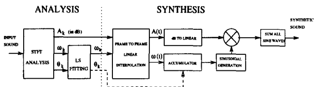
Figure 2: A block diagram of the complete analysis/synthesis system. Note that the fitted phase samples that need not be saved (or transmitted) are denoted by a dashed line.
