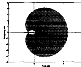
Figure 1: Unit circle inside the convergence domain of LIF.
