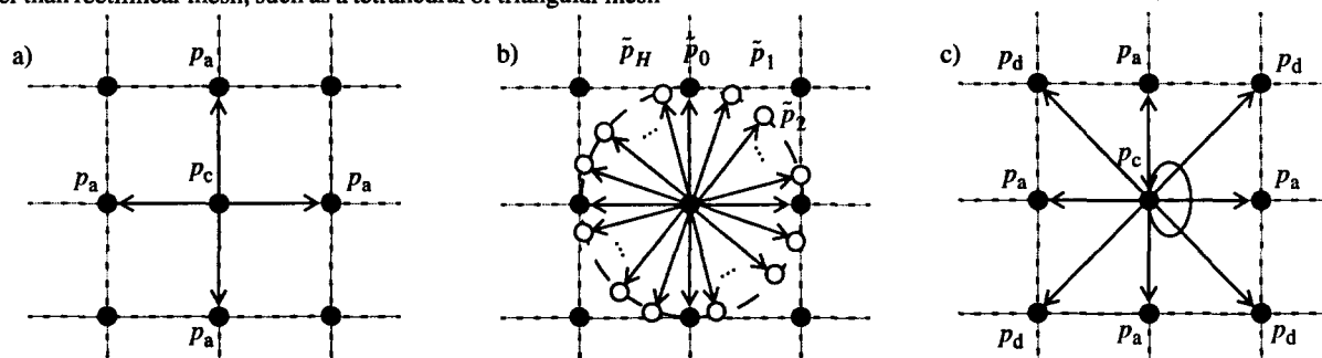
Figure 1: 2D waveguide mesh structures: a) the original mesh with 4 directions, b) the hypothetical version with H propagation directions, c) the new deinterpolated waveguide mesh, where the new \tilde{p}_h nodes are spread onto the neighboring nodes by deinterpolation.
