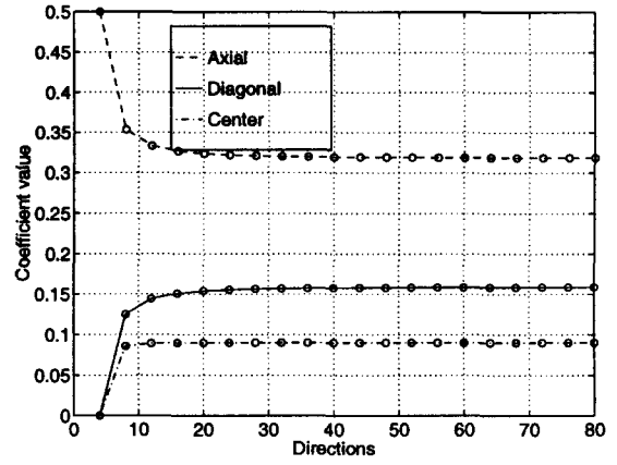
Figure 3: Weighting coefficients h_d, h_a, h_c as function of number of wave propagation directions.
