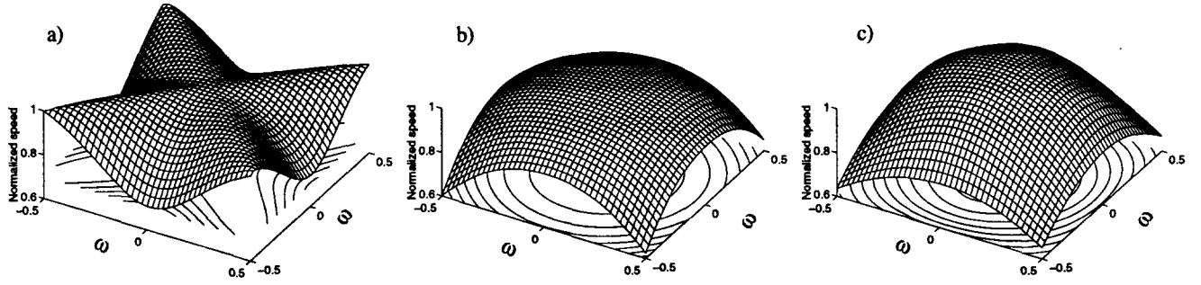
Figure 4: Normalized wave travel speeds in a) the original, b) the hypothetical 8-directional, and c) the deinterpolated 8-directional waveguide mesh structures as a function of normalized frequency.
