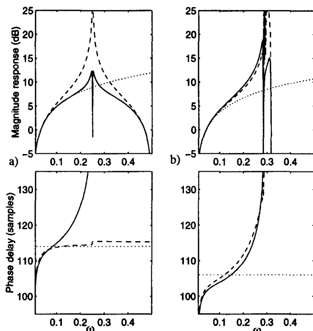
Figure 5: Magnitude responses and phase delays to axial (—) and diagonal(---) directions in a) original, and b) deinterpolated 8-directional waveguide mesh structures. Dotted line (..) represents the ideal response in each case.
