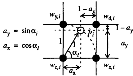
Figure 2: Bilinear deinterpolation coefficients are calculated from this geometry.
