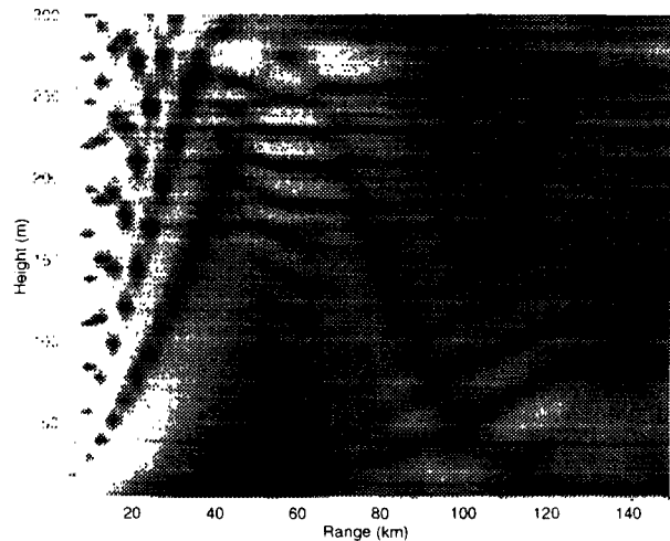
Figure 2. Coverage diagram showing propagation loss as a function of height and range for the tri-linear refractivity profile, RF emitter at 50 m, the frequency is 1 GHz. The transmission loss scale is from less than 100 dB (white) to greater than 150 dB (black).
