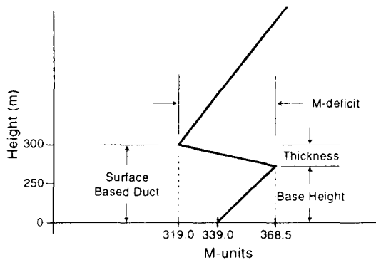
Figure 1. Modified vertical refractivity for a tri-linear profile.
