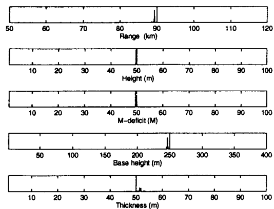
Figure 5. GA estimated a posteriori distributions for source range, source height, M-deficit, base-height, and layer thickness, antenna aperture was 98 m.
