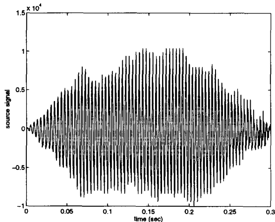
Figure 4. Segment of a whale call.
