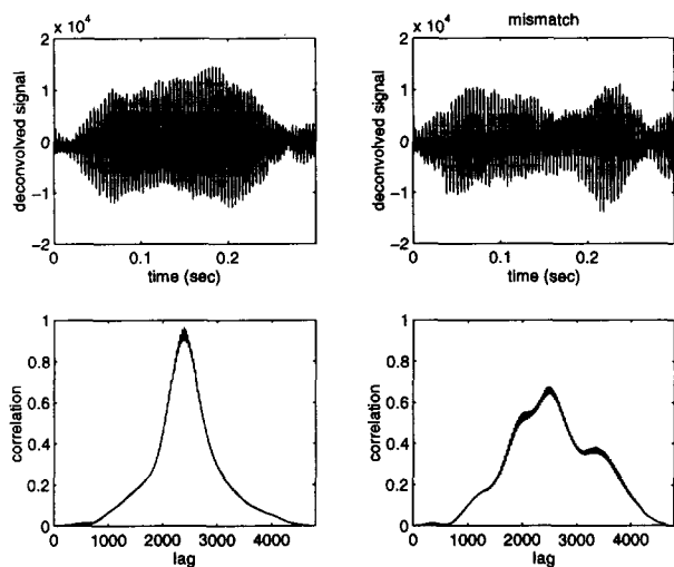
Figure 5. Deconvolved signals and correlations between the deconvolved signals and the originally transmitted whale call.
