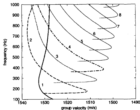
Figure 1. Dispersion curves for the propagation medium.
