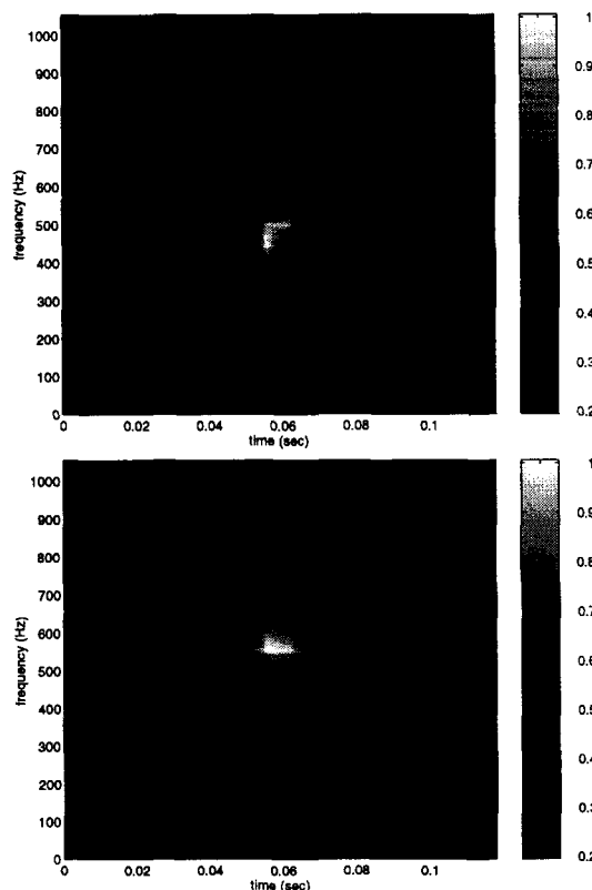
Figure 2. Spectrograms of the transmitted and received pulses.
