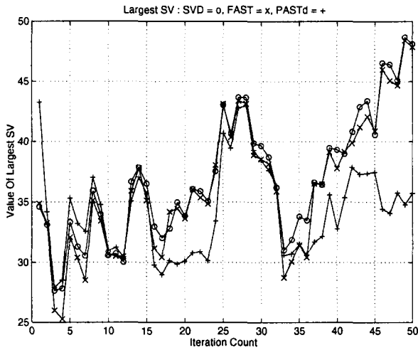
Figure 1: A comparison of the trace of the largest singular value computed by the SVD over 50 iterations vs. the estimate of it from the various algorithms indicated.
