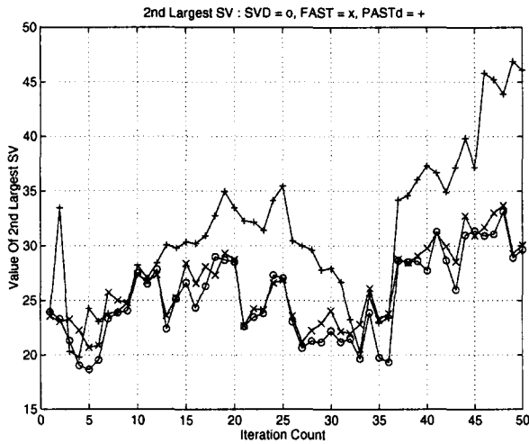
Figure 2: A comparison of the trace of the second largest singular value computed by the SVD over 50 iterations vs. the estimate of it from the various algorithms indicated.
