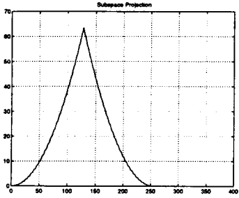
Figure 3: Subspace Projection
