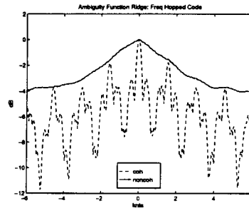
Figure 6: Ambiguity Ridge
