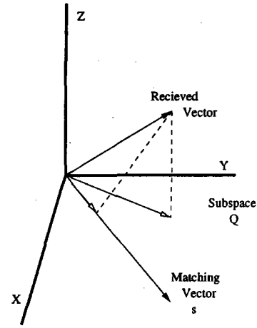
Figure 1: Projection Subspace
