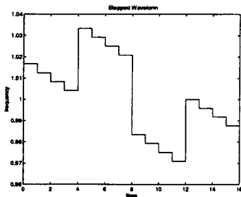
Figure 4: Waveform
