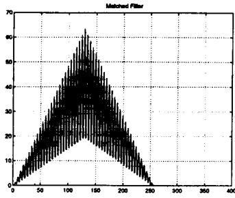
Figure 2: Standard Autocorrelation
