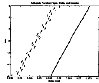
Figure 5: Ridge
