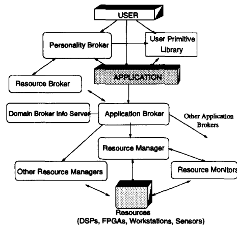
Figure 3. Architecture of Brokered Computation Model
