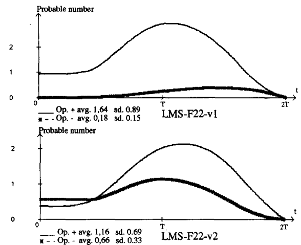
Figure 5. Estimations of Add. and sub. number for the LMS-F22 algo. with 2048 taps
