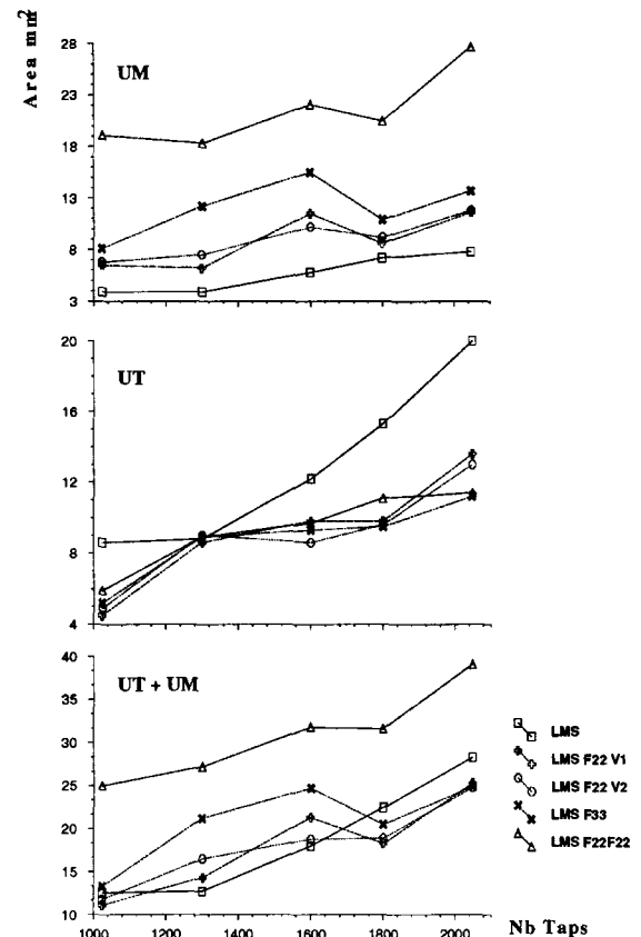
Figure 4. LMS cost vs taps
