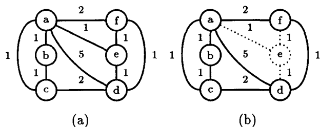
Figure 3: (a) Access graph, (b) heuristic extension of partial layout \varphi_1 = b\langle ac \rangle to \varphi_2 = bcadf .
