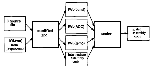
Figure 4. Overall Compiler structure
