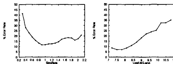
Figure 1. Error rate over feature value for feature T-active-Leaf (right) and feature SpkRate (left)
