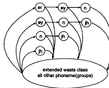
Figure 4: Speech model for calculations on parts of the keyword "er_ey_n_jh" e.g. "er_ey" and "jh"
