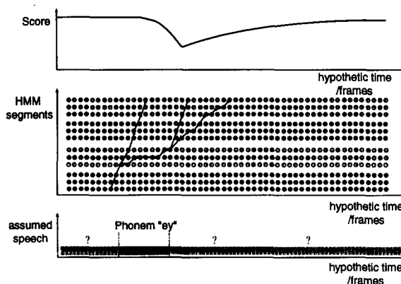
Figure 3: Score and model trellis for of phoneme "ey" matching
