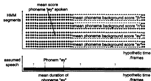
Figure 2: Model trellis for the keyword "er_ey_n_jh"
