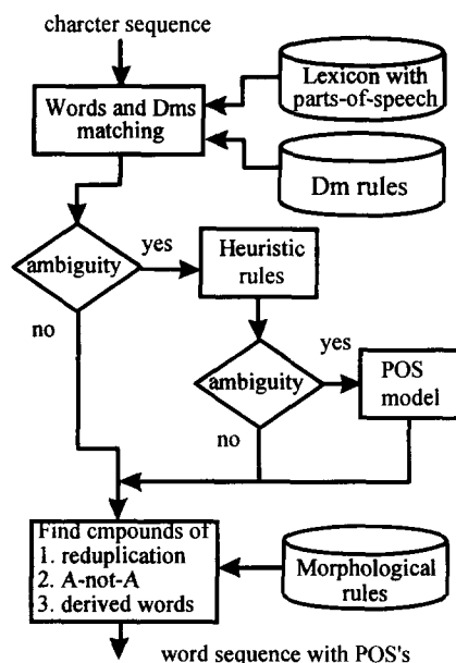
Figure 1: The diagram for word identification and tagging.
