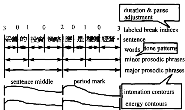
Figure 2: The mechanism for the determination of the prosodic parameters according to the prosodic structure.
