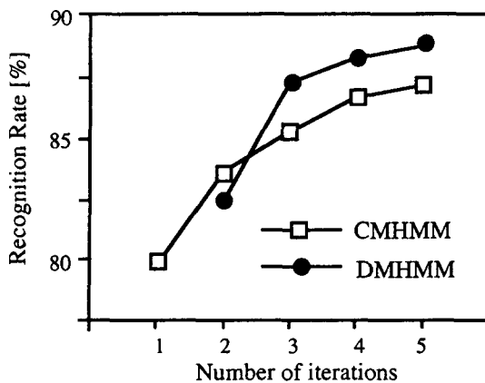
Figure 4. Recognition rates along with training iterations.
