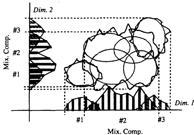
Figure 3. Feature parameter space represented by a discrete mixture HMM (DMHMM).
