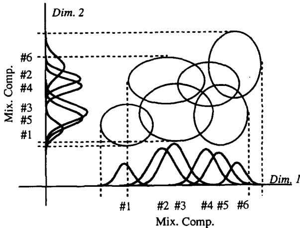
Figure 2. Feature parameter space represented by a continuous mixture HMM (CMHMM).
