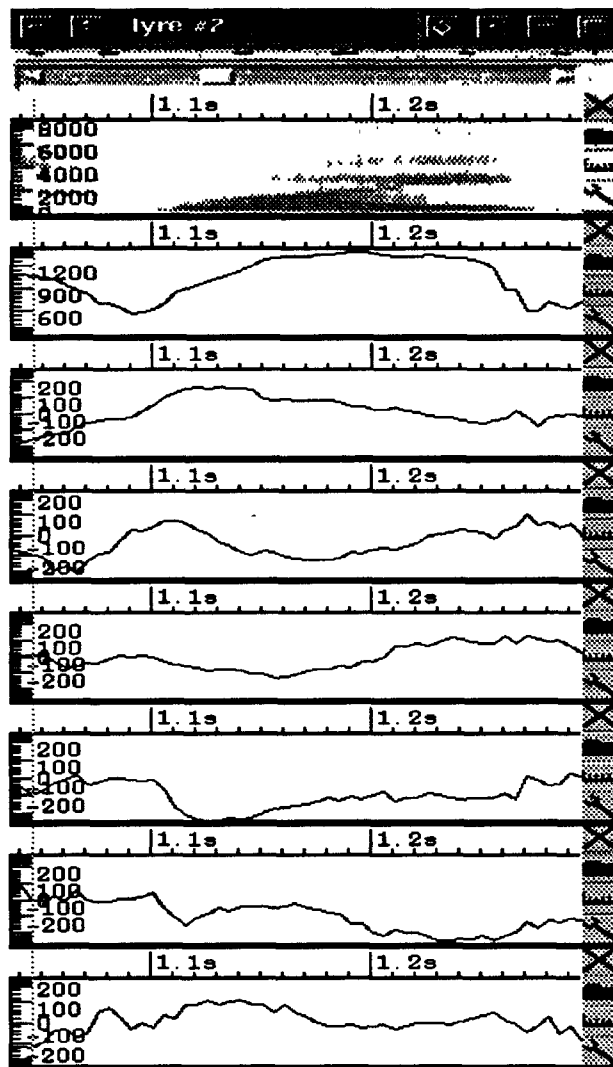
Figure 2. Spectrogram and the MFCC trajectories of signal for a TIMIT example (phoneme "ay").
