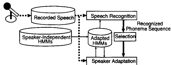
Figure 6. Iterative unsupervised speaker adaptation procedure
