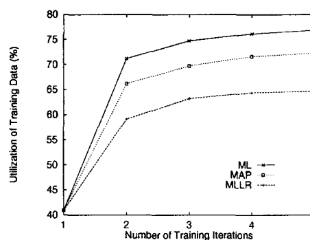
Figure 8. Utilization of training data in iterative unsupervised speaker adaptation with new supervision selection method
