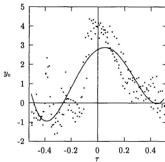
Figure 2. First cepstral coefficients of word ZWEI and polynomial approximation
