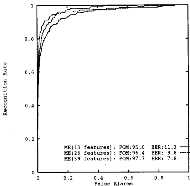
Figure 5: ROC curves showing relative performance of System with and without Delta and Delta-delta cepstra, Means Estimated models with 120s Training. One-session, 10s test.
