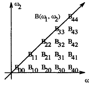
Figure 1. First 15 points in the nonredundant region of the bispectrum.
