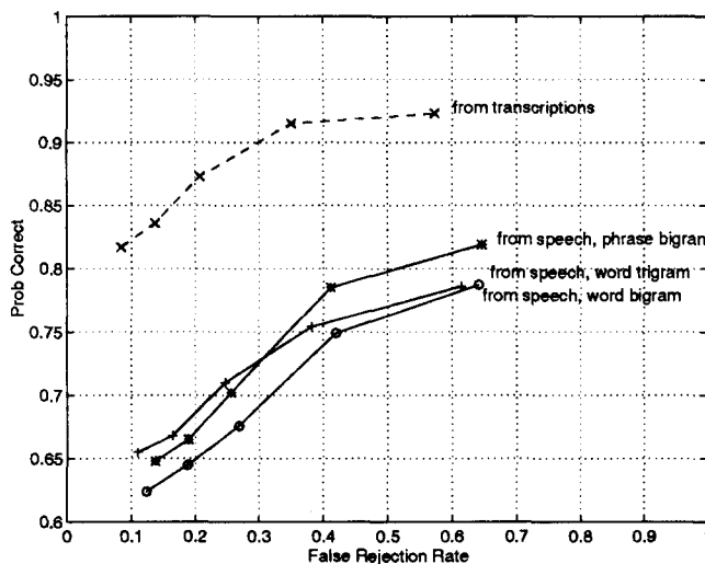
Figure 4: Rank 1 classification rate from text and speech with word n -grams and phrase bigrams
