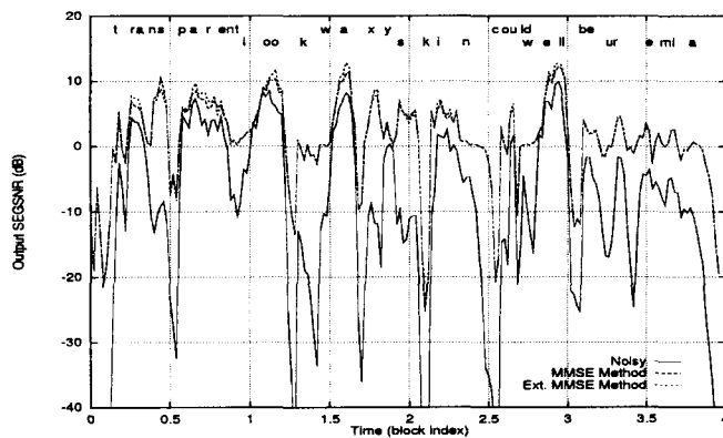
Figure 1. Segmental SNR at 0 dB input SNR for a female speaker.
