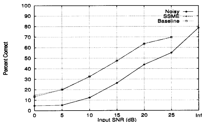
Figure 2. Alphabet recognition performance.
