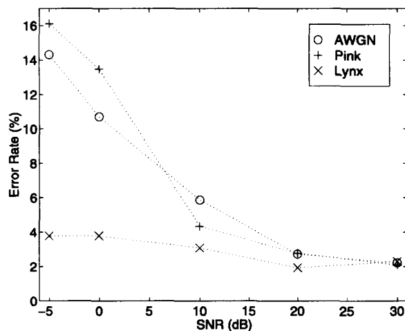
Figure 1. Performance of SPD-MAP.
