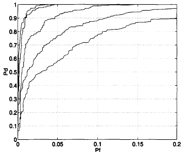
Figure 3. Receiver Operating Curves of SPD-NP in AWGN at input SNRs of 30, 20, 10, 0 and -5 dB.
