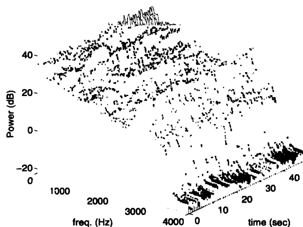
Figure 4. Spectrogram of F16 noise from NOISEX-92.
