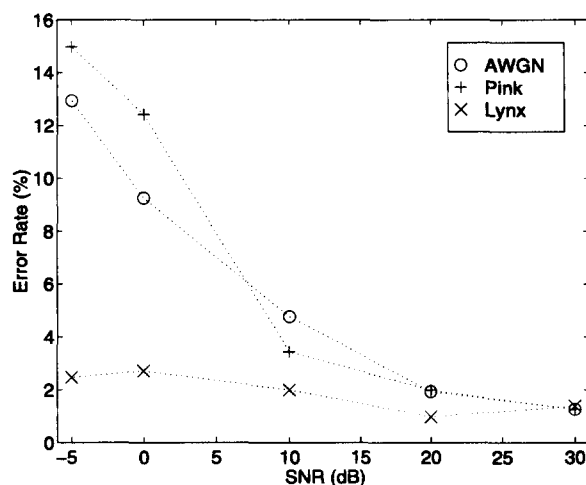
Figure 2. Performance of SPD-MAP, excluding transition frames.
