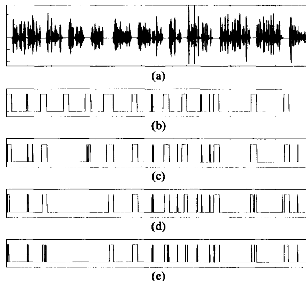
Figure 5. Operation of SPD-NP ( \eta=0.4 ) in non-stationary F16 noise. (a) 11 sentences of speech with no noise; (b) manually identified pauses; (c)-(e) SPD-NP at input SNRs of 10, 0 and -5 dB, respectively.
