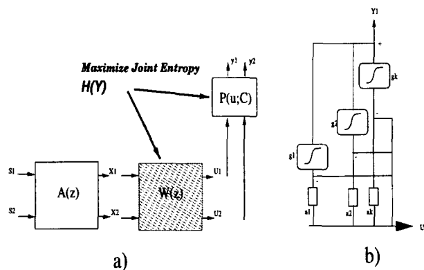
Figure 1. a) A(z) denotes the mixing system and W(z) denotes the unmixing system. W(z) can be a feedback or a feedforward architecture. b) Contextual density estimation as a sum of nonlinearities
