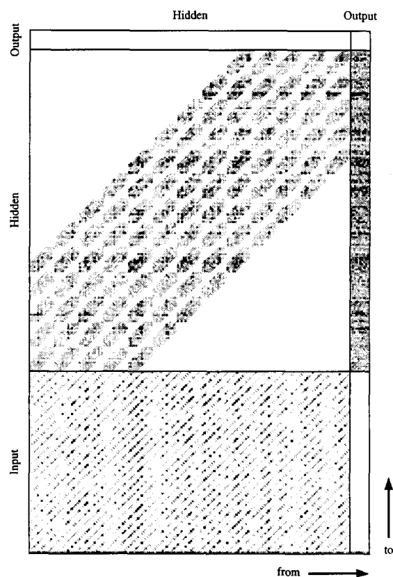
Figure 2. Weight values of a LRNN based on PEMO processing for recognition of 10 digits
